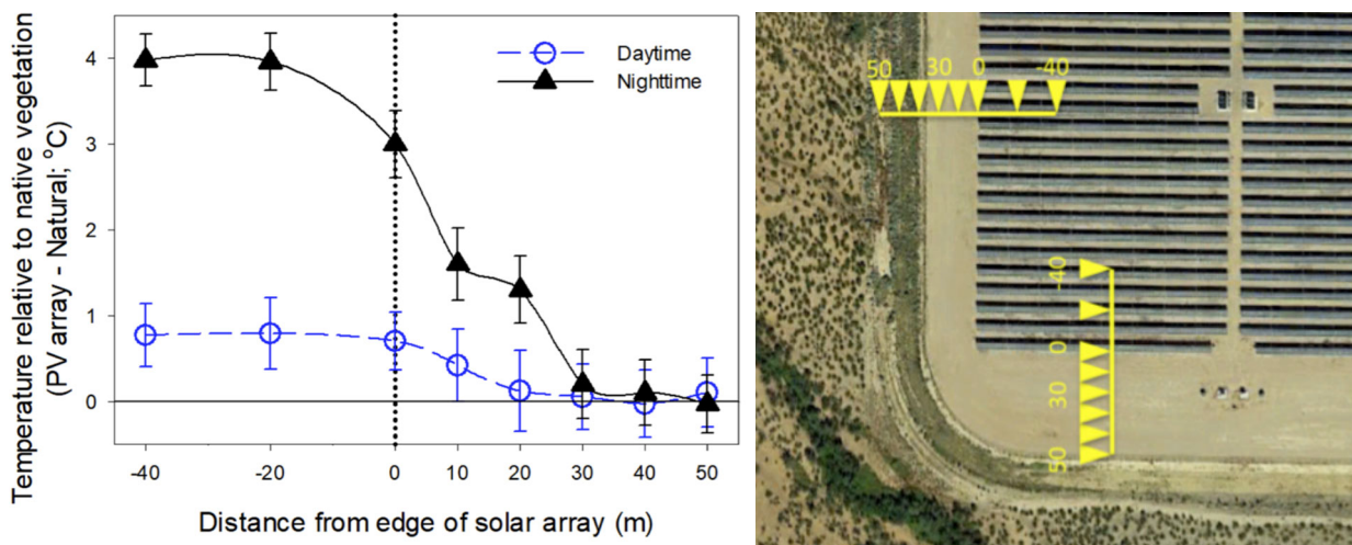
Fig 2. The small temperature increases observed at an unvegetated desert project was negligible within 100 ft of the edge of the solar array
